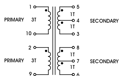
Transformer schematic
